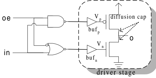
Figure 3 Circuit diagram of tri-state bus driver.
