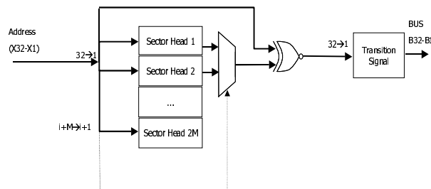
Figure 4- FMS Encoder
