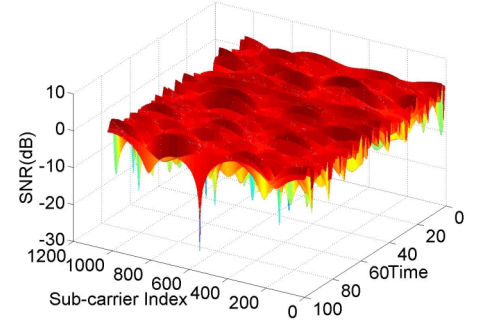
(a) Actual channel characteristics
