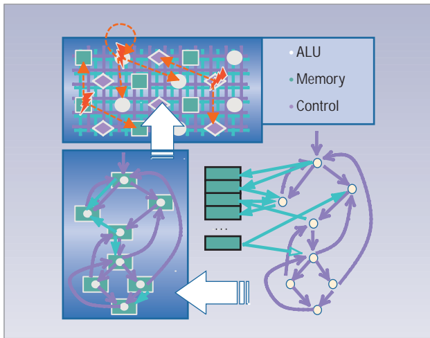
Figure 4. Possible architectural path. The design progresses from program description to regular tile-based processor nanoarchitectures.
