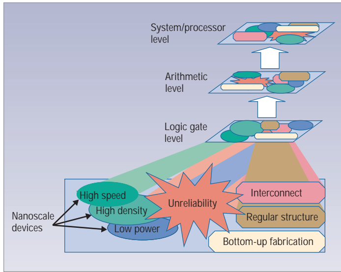
Figure 2. Nanosystem opportunities and attributes. Nanoelectronics will shape design approaches at various levels of abstraction.
