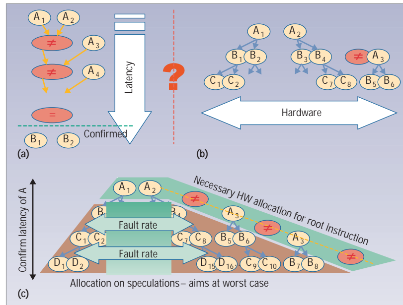
Figure 1. Nanosystem reliability. Temporal (a) and hardware (b) redundancy have traditionally resolved high fault rates. (c) Hybrid architectures necessitate exploration of a speculation-based adaptive mode.
