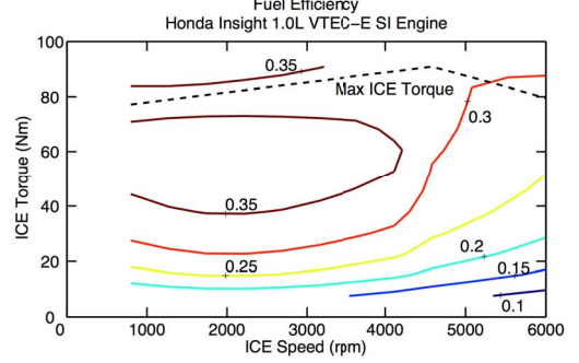
Figure 2. Fuel efficiency map of an ICE.
