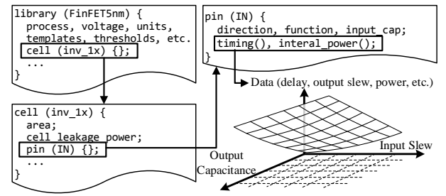
Figure 2. Hierarchy of Liberty format library.
