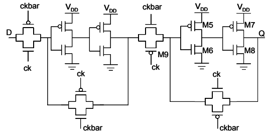
Figure 8. Negative-edge triggered master-slave flip-flop.
