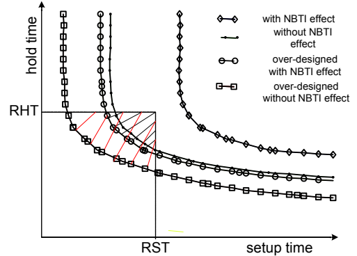
Figure 7. Flip-flop design.
