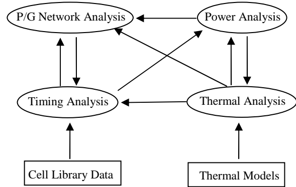
Figure 7: Thermal analysis affects timing (with signal integrity), power and P/G network analyses.
