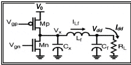
Figure 3 The Buck Converter of a DC/DC converter.
