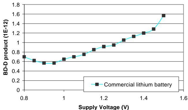
Figure 9 Experimental results of the BD - D product curve.
