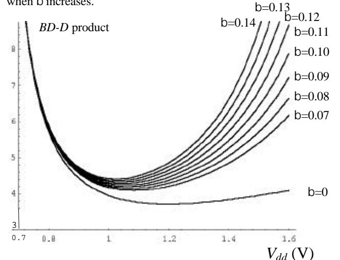
Figure 8 BD - D product curves with different b values (VOL).
