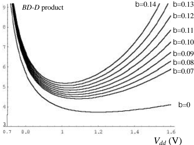
Figure 7 BD - D product curves with different b values (FOL).
