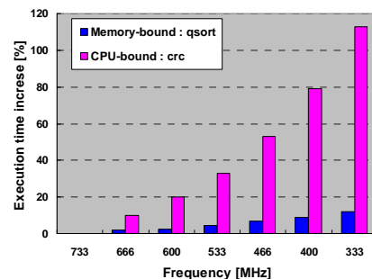
Figure 1: Execution time changes according to CPU frequency
