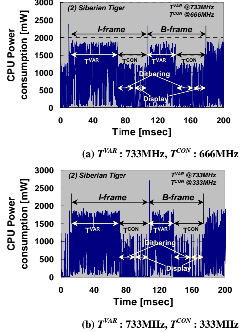
Figure 7: Decoding time and power consumption at different CPU frequencies and voltage levels
