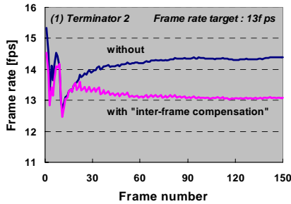
Figure 10: Frame rate variation with the proposed DVFS
